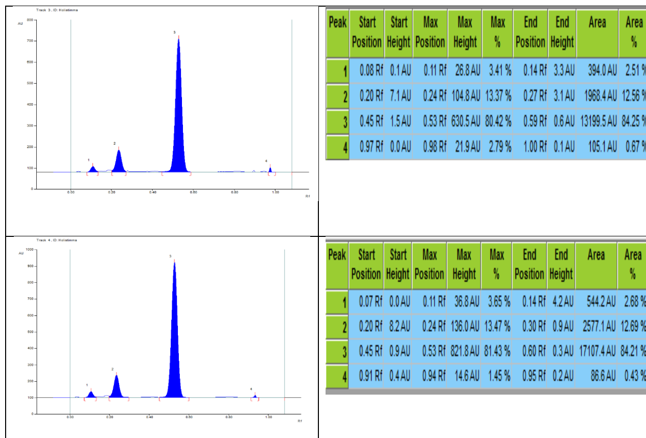
Figure 4. Densitogram, Rf values and peak area showing percentage of secondary metabolites in methanolic root tuber extract under 15 \mu l and 20 \mu l of Holostemma ada-kodien at 366 nm.
