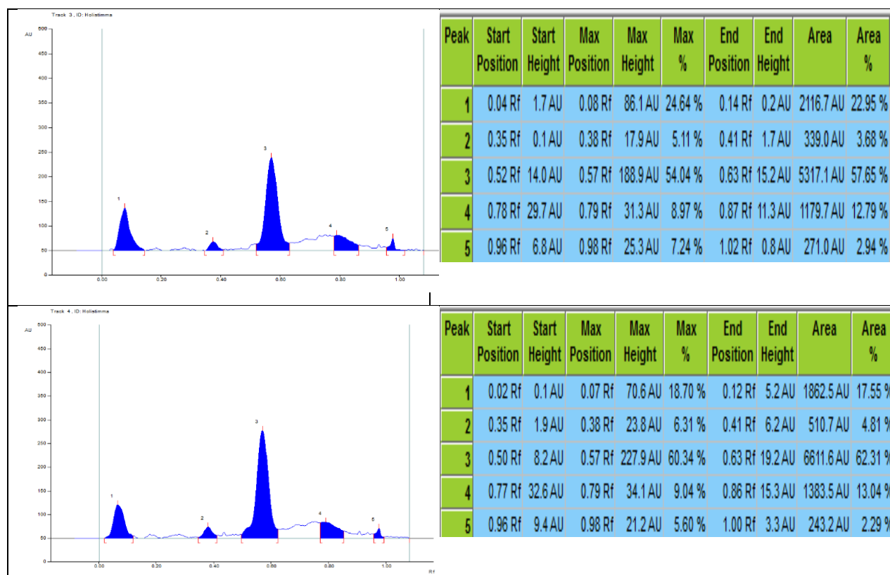
Figure 3. Densitogram, Rf values and peak area showing percentage of secondary metabolites in methanolic root tuber extract under 15 \mu l and 20 \mu l of Holostemma ada-kodien at 254 nm.
