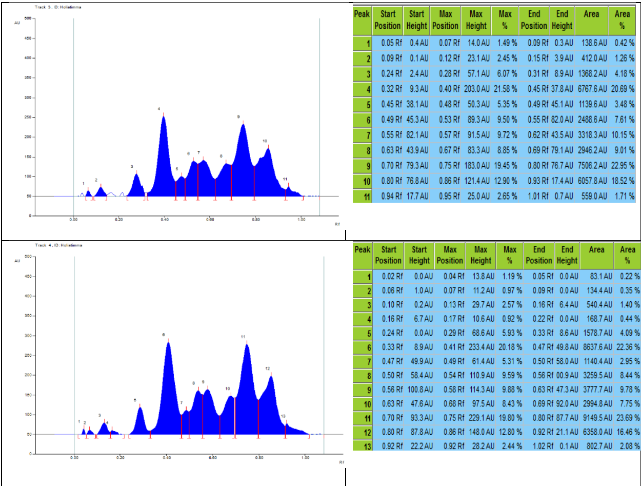
Figure 5. Densitogram, Rf values and peak area showing percentage of secondary metabolites in methanolic root tuber extract under 15 µl and 20 µl of Holostemma ada-kodien at 575 nm.
