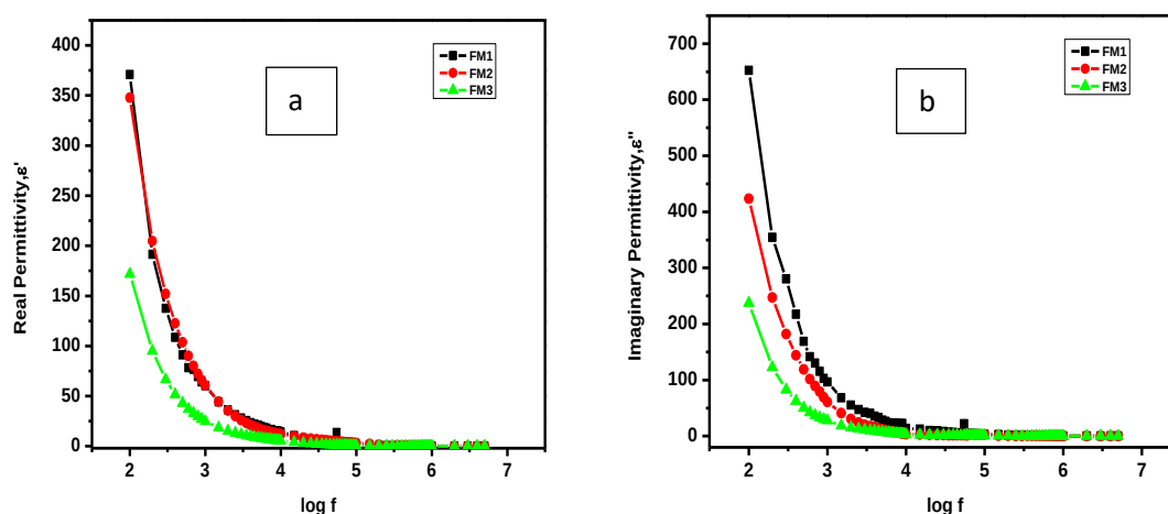
Figure 5. Variation of real and imaginary permittivity with frequency at different concentration shown in (i) a and (ii) b
