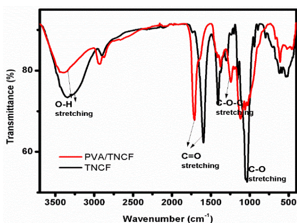
Figure 9. ATR FT-IR spectrum of PVA-TNCF aerogel.
